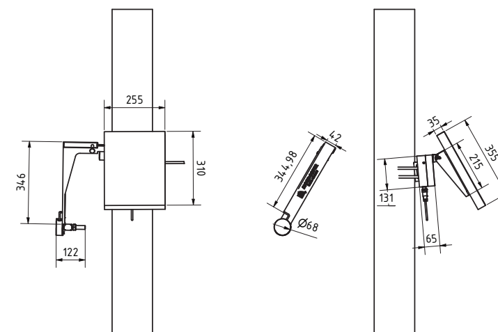
Front view (Dimension MM (NTS))
